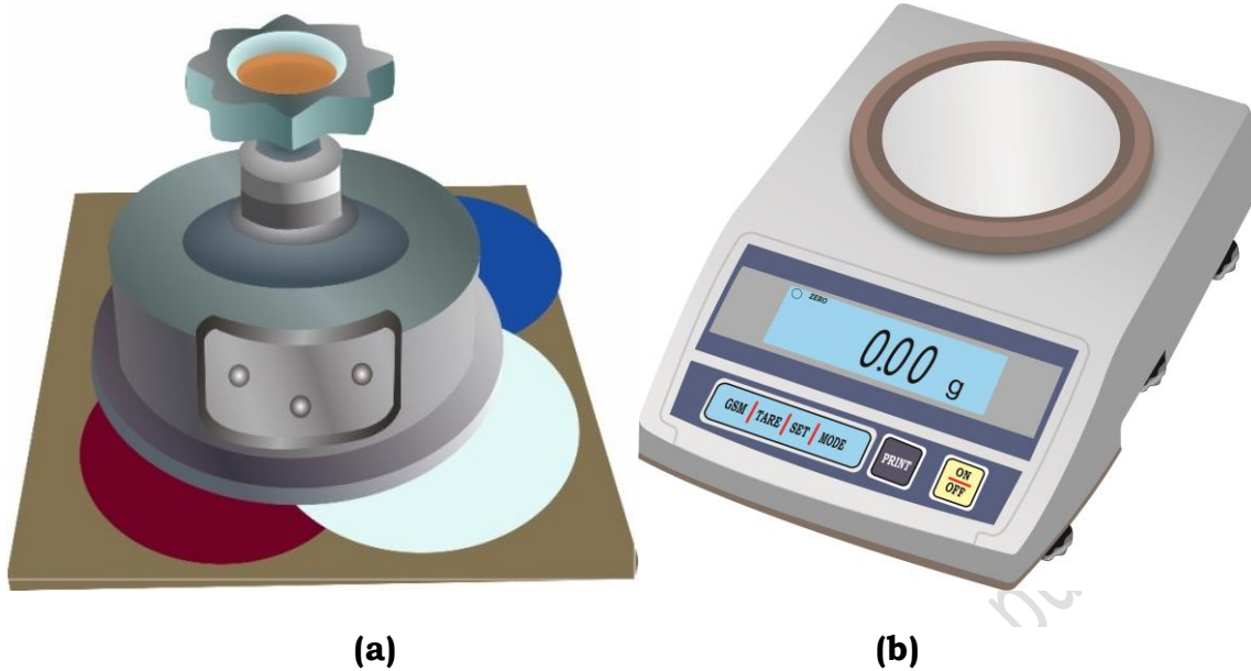
Fig. 1.4(a & B) : GSM cutter and weighing balance
